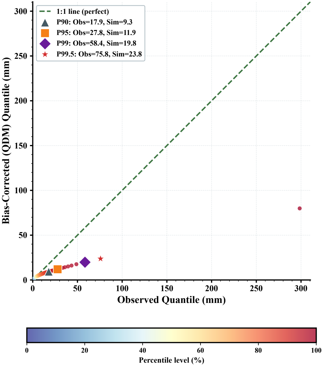
(b) Observed vs Bias-Corrected (QDM) QQ-RMSE = 17.02 mm
