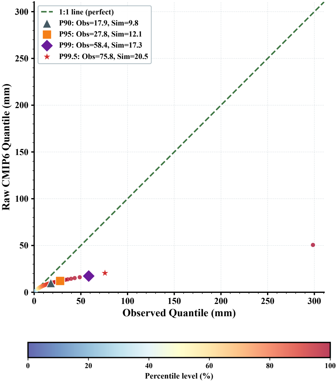
(a) Observed vs Raw CMIP6 QQ-RMSE = 18.98 mm
